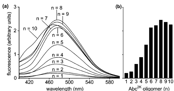
Figure 2. FRET study of peptides 10a–j: (a) fluorescence emission spectra of 1.75 μM solutions of the peptides in 50% aqueous DMSO solution with 335 nm excitation; (b) fluorescence intensity at λ max .
